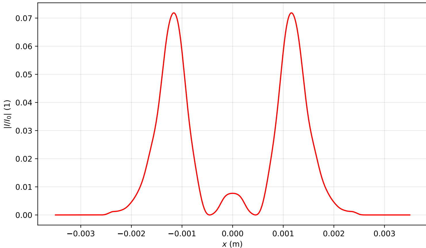
Intensity profile I(x, y = 0, z = 3.582)/I_0 , P_{in}=7.5P_{cr} , artificial time
